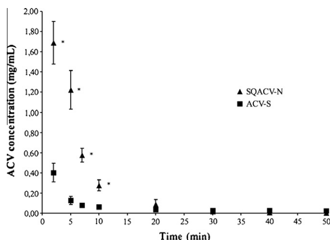
Fig. 3. Tear fluid concentration vs time profiles of ACV after administration of (▲) SQACV-N (total-ACV) and (■) ACV-S (intact-ACV) formulations. (Means \pm S.E., n = 6 , *: significantly different from ACV-S ( p < 0.05 )).
