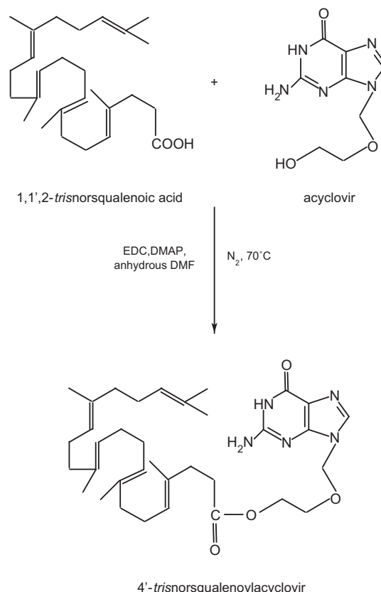
Fig. 1. Reaction scheme for the synthesis of 4'-trisnorsqualenoylacyclovir.
