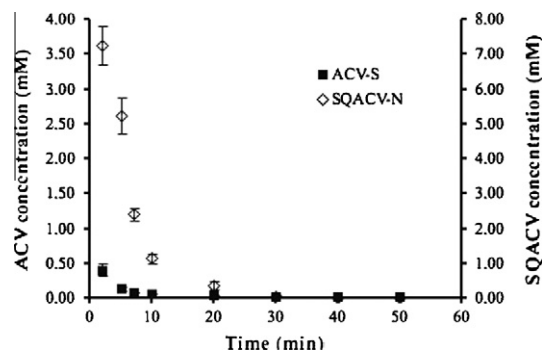
Fig. 2. Tear fluid concentration vs time profiles of ACV and SQACV upon topical administration of (■) reference ACV aqueous solution (ACV-S) and (◇) SQACV nanoassemblies (SQACV-N) formulations, respectively. (Means \pm S.E., n = 6 ).
